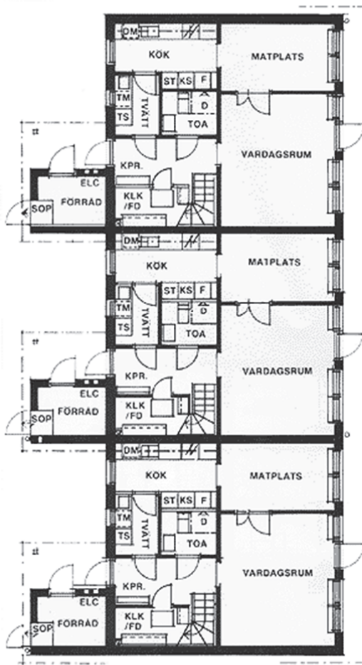
Bottenplan
